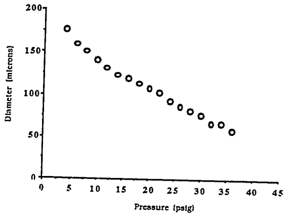
Figure 6. PDPA Data - Sauter Mean Diameter
