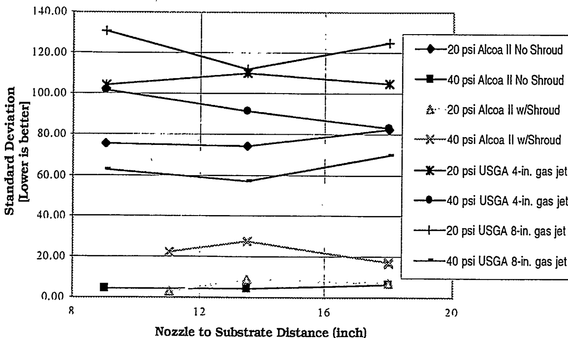
Figure 9. Effect of Nozzle Geometry and Process Parameters on the Deposit Profile Flatness.
